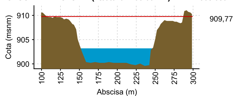
CAUCA - LA VICTORIA (28/09/2022 06:00 AM) NIVEL: 903.089
