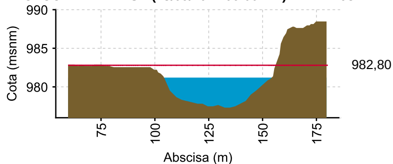
CAUCA - LA Balsa (28/09/2022 06:00 AM) NIVEL= 981.1
