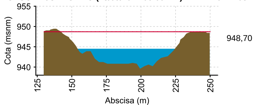
CAUCA - JUANCHITO (28/09/2022 06:00 AM) NIVEL= 944.403
