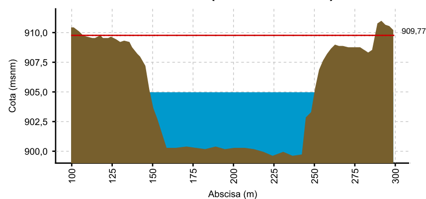
CAUCA - LA VICTORIA (02/09/2021 06:00 AM) NIVEL= 904.939
