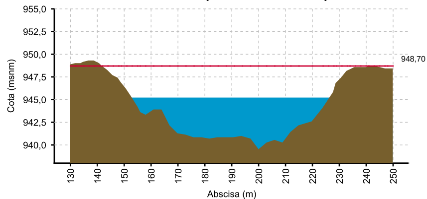
CAUCA - JUANCHITO (02/09/2021 06:00 AM) NIVEL= 945.183
