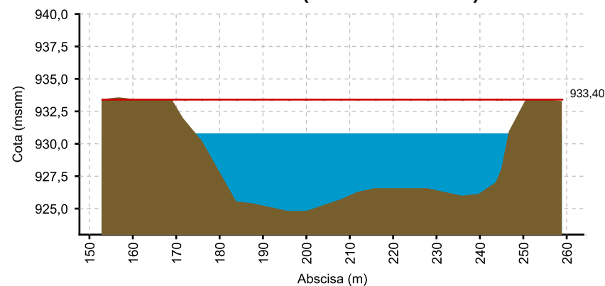
CAUCA - MEDIACANOA (02/09/2021 06:00 AM) NIVEL= 930.754
