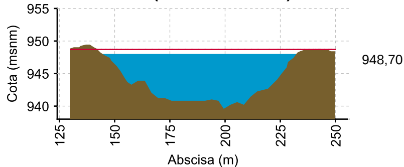
CAUCA - JUANCHITO (28/10/2022 04:00 PM) NIVEL= 948.003
