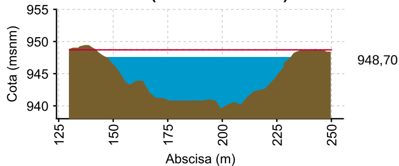
CAUCA - JUANCHITO (24/11/2022 06:00 AM) NIVEL= 947.443
