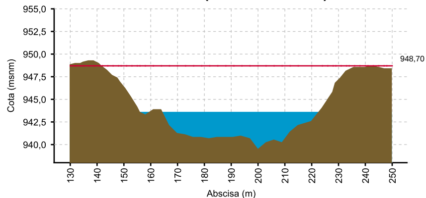
CAUCA - JUANCHITO (21/05/2020 06:00 AM) NIVEL= 943.563
