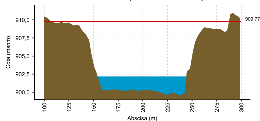
CAUCA - LA VICTORIA (21/05/2020 06:00 AM) NIVEL: 902.149
