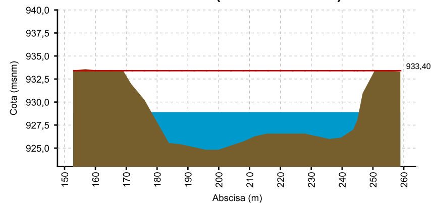
CAUCA - MEDIACANOA (21/05/2020 06:00 AM) NIVEL= 928.774
