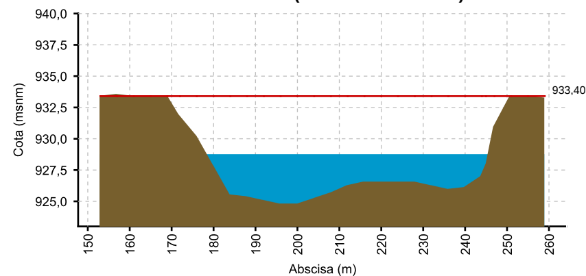
CAUCA - MEDIACANOA (17/05/2020 06:00 AM) NIVEL= 928.724
