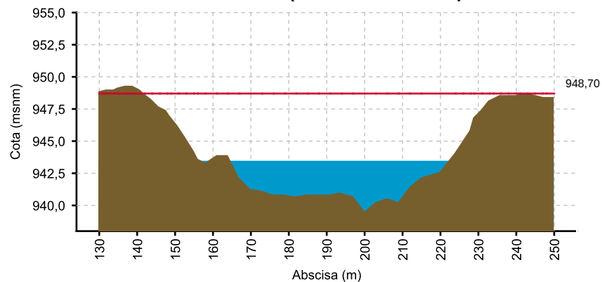
CAUCA - JUANCHITO (17/05/2020 06:00 AM) NIVEL= 943.463
