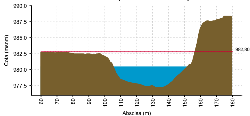
CAUCA - LA BALSA (17/05/2020 06:00 AM) NIVEL= 980.49
