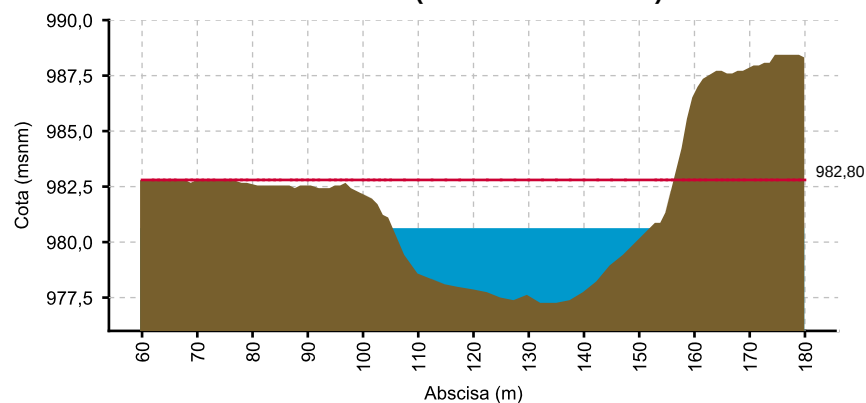
CAUCA - LA BALSA (16/05/2020 06:00 AM) NIVEL= 980.6
