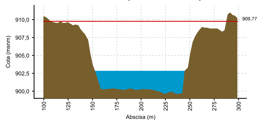
CAUCA - LA VICTORIA (16/05/2020 06:00 AM) NIVEL: 902.809
