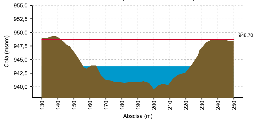
CAUCA - JUANCHITO (15/05/2020 06:00 AM) NIVEL= 943.763
