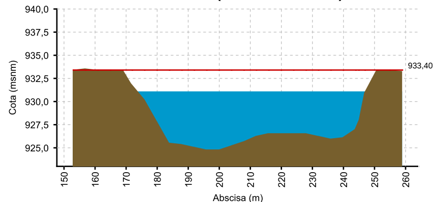
CAUCA - MEDIACANOA (27/06/2021 06:00 AM) NIVEL= 930.964
