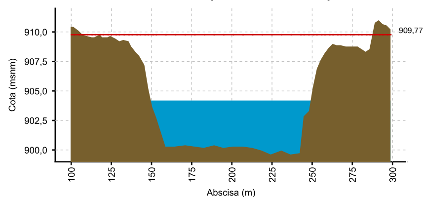
CAUCA - LA VICTORIA (27/06/2021 06:00 AM) NIVEL= 904.189
