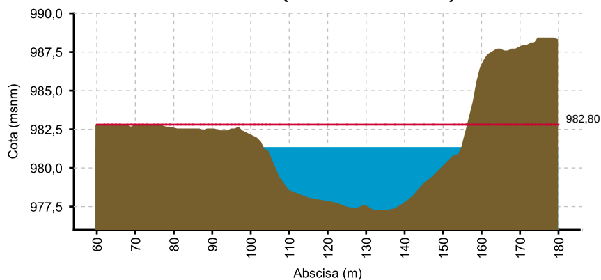
CAUCA - LA BALSA (27/06/2021 06:00 AM) NIVEL= 981.29
