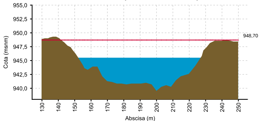
CAUCA - JUANCHITO (27/06/2021 06:00 AM) NIVEL= 945.403
