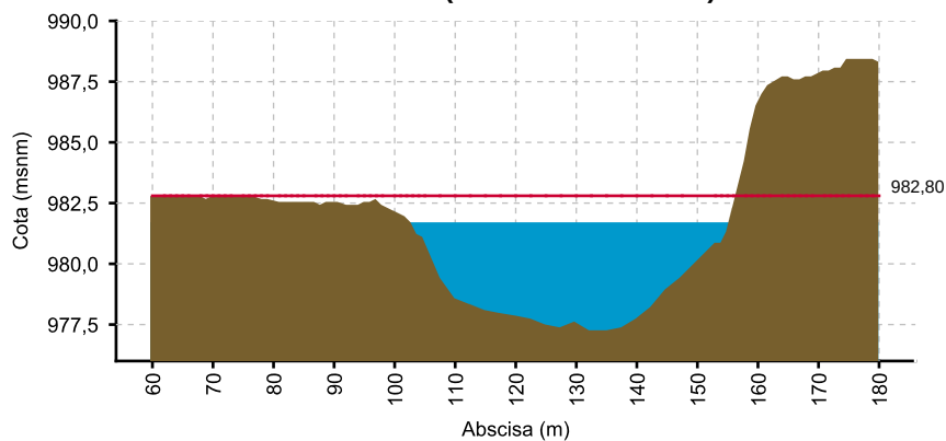
CAUCA - LA BALSA (09/06/2021 06:00 AM) NIVEL= 981.69
