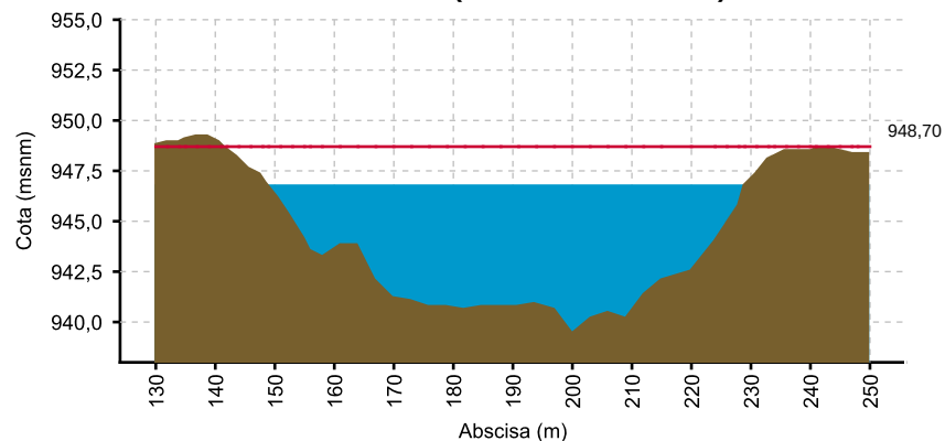
CAUCA - JUANCHITO (08/06/2021 06:00 AM) NIVEL= 946.743
