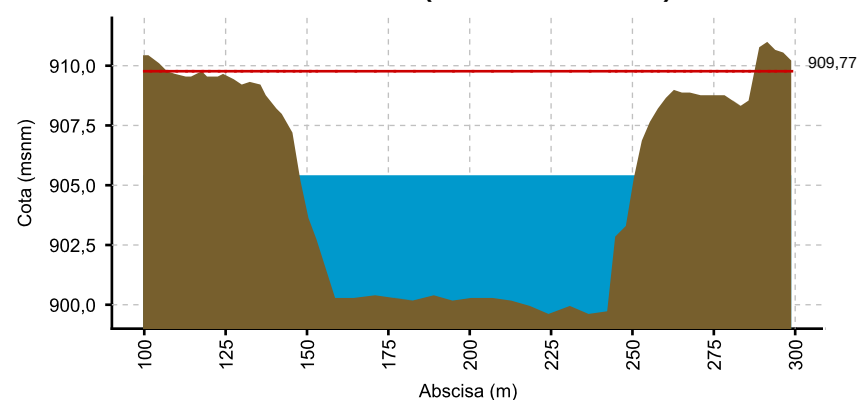
CAUCA - LA VICTORIA (08/06/2021 01:00 AM) NIVEL: 905.329
