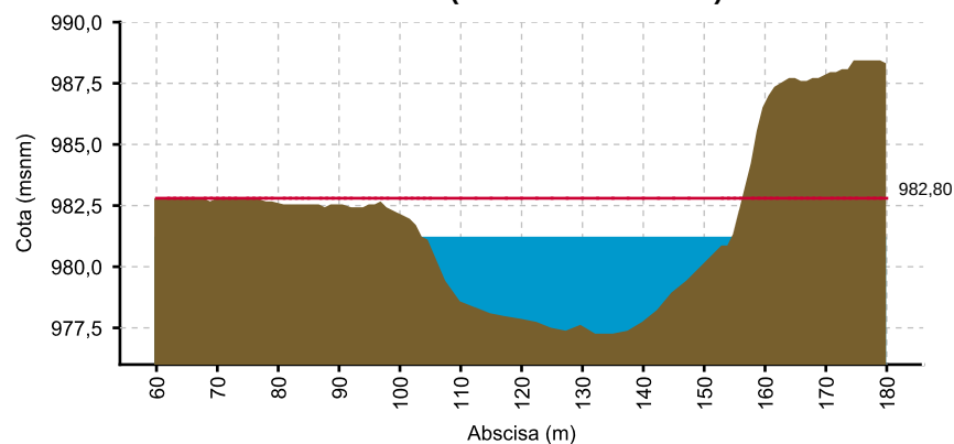
CAUCA - LA BALSA (03/06/2021 06:00 AM) NIVEL= 981.22
