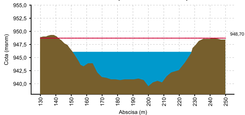
CAUCA - JUANCHITO (03/06/2021 06:00 AM) NIVEL= 945.963
