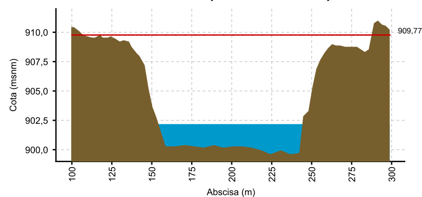
CAUCA - LA VICTORIA (30/07/2020 06:00 AM) NIVEL: 902.169
