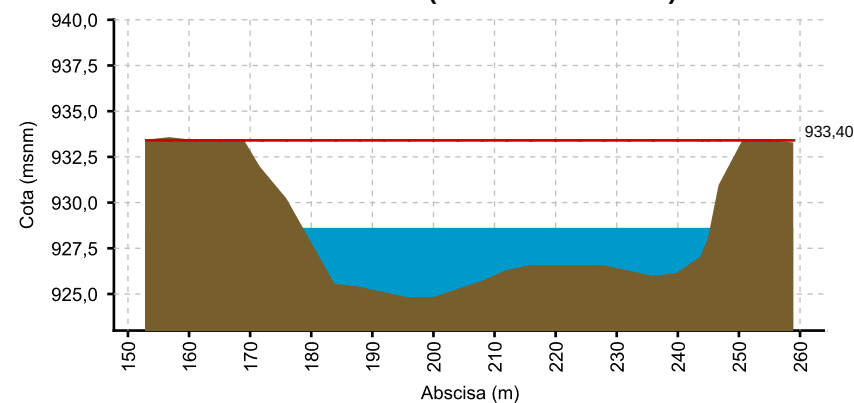
CAUCA - MEDIACANOA (30/07/2020 06:00 AM) NIVEL= 928.604
