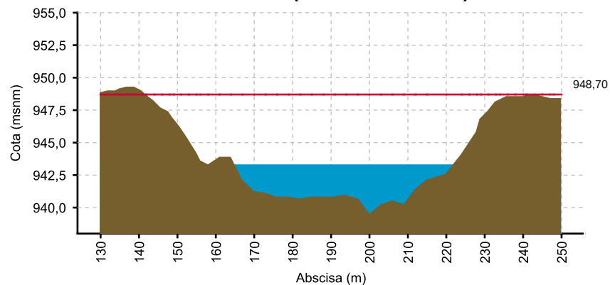
CAUCA - JUANCHITO (29/07/2020 06:00 AM) NIVEL= 943.303
