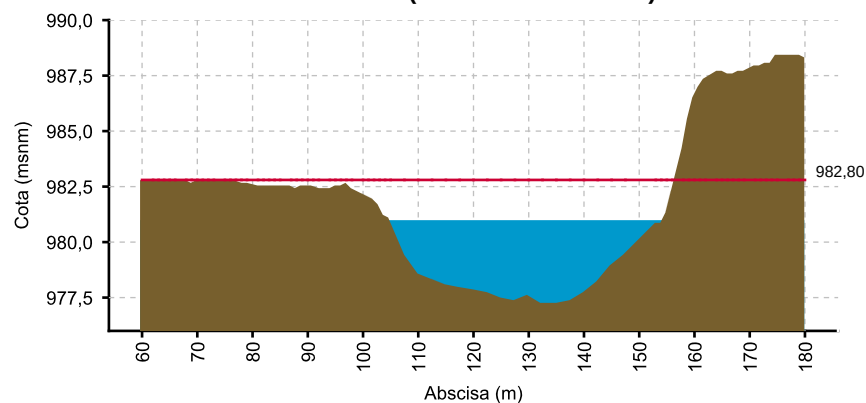
CAUCA - LA BALSA (30/07/2020 06:00 AM) NIVEL= 980.88
