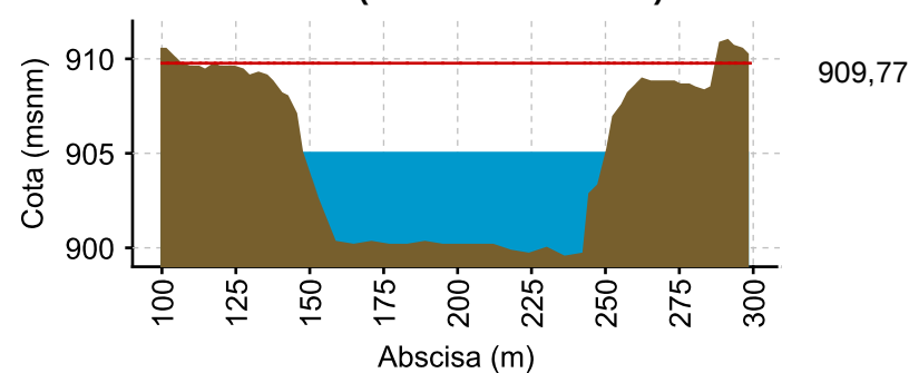
CAUCA - LA VICTORIA (19/12/2022 04:00 PM) NIVEL: 905.069
