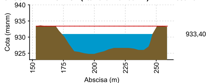
CAUCA - MEDIACANOA (19/12/2022 04:00 PM) NIVEL= 930.794
