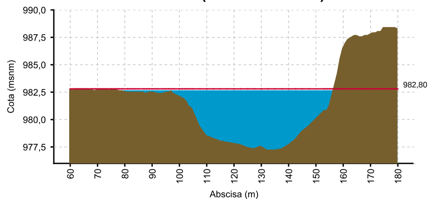
CAUCA - LA BALSA (26/08/2021 06:00 AM) NIVEL= 982.59
