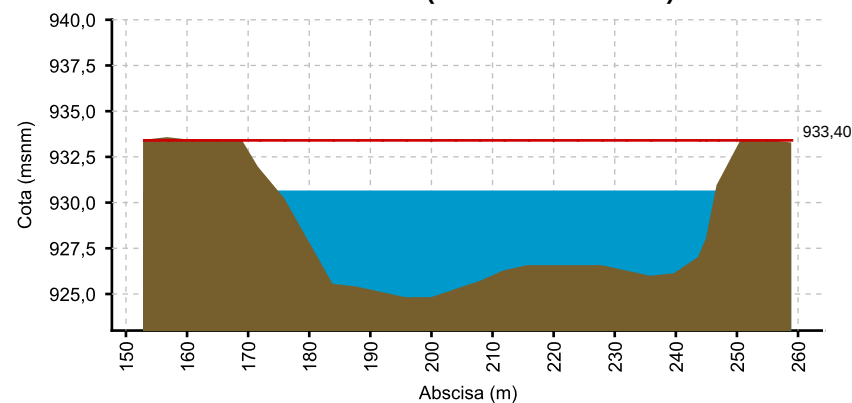
CAUCA - MEDIACANOA (26/08/2021 06:00 AM) NIVEL= 930.654
