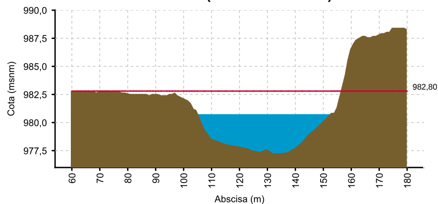
CAUCA - LA BALSA (17/04/2020 06:00 AM) NIVEL= 980.63
