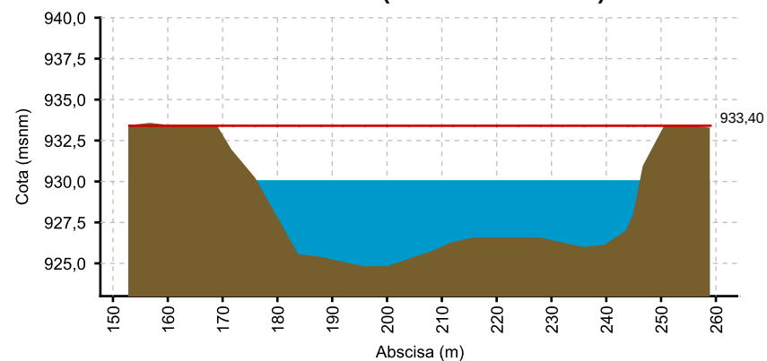
CAUCA - MEDIACANOA (17/04/2020 06:00 AM) NIVEL= 930.074
