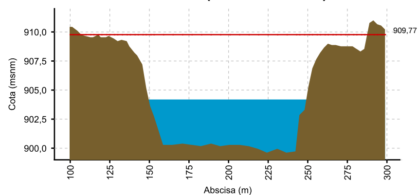
CAUCA - LA VICTORIA (17/04/2020 06:00 AM) NIVEL: 904.079
