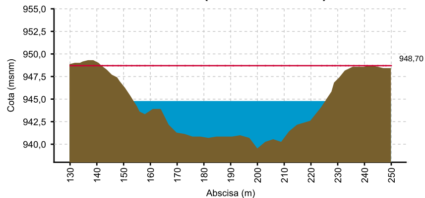
CAUCA - JUANCHITO (17/04/2020 06:00 AM) NIVEL= 944.643
