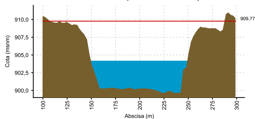
CAUCA - LA VICTORIA (16/04/2020 06:00 AM) NIVEL: 904.179
