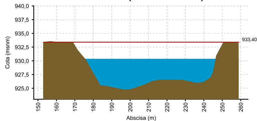
CAUCA - MEDIACANOA (16/04/2020 06:00 AM) NIVEL= 930.274
