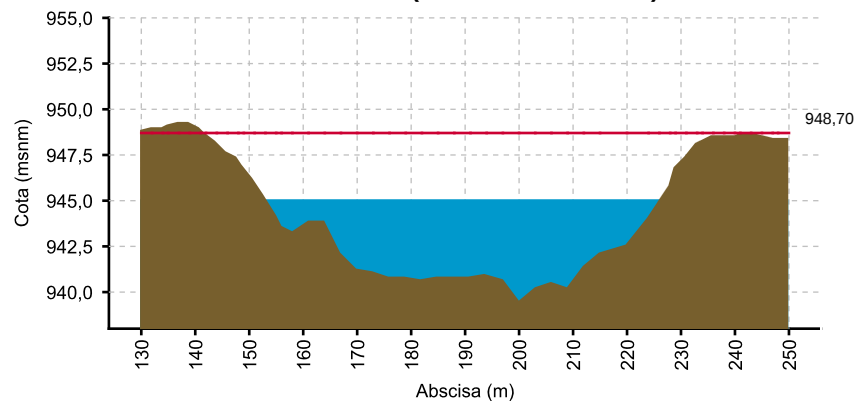
CAUCA - JUANCHITO (16/04/2020 06:00 AM) NIVEL= 944.983
