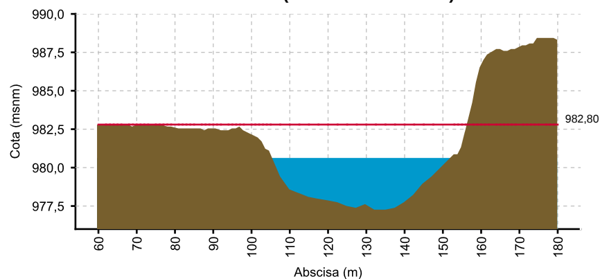
CAUCA - LA BALSA (16/04/2020 06:00 AM) NIVEL= 980.58
